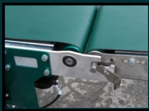
Quick-attach system
